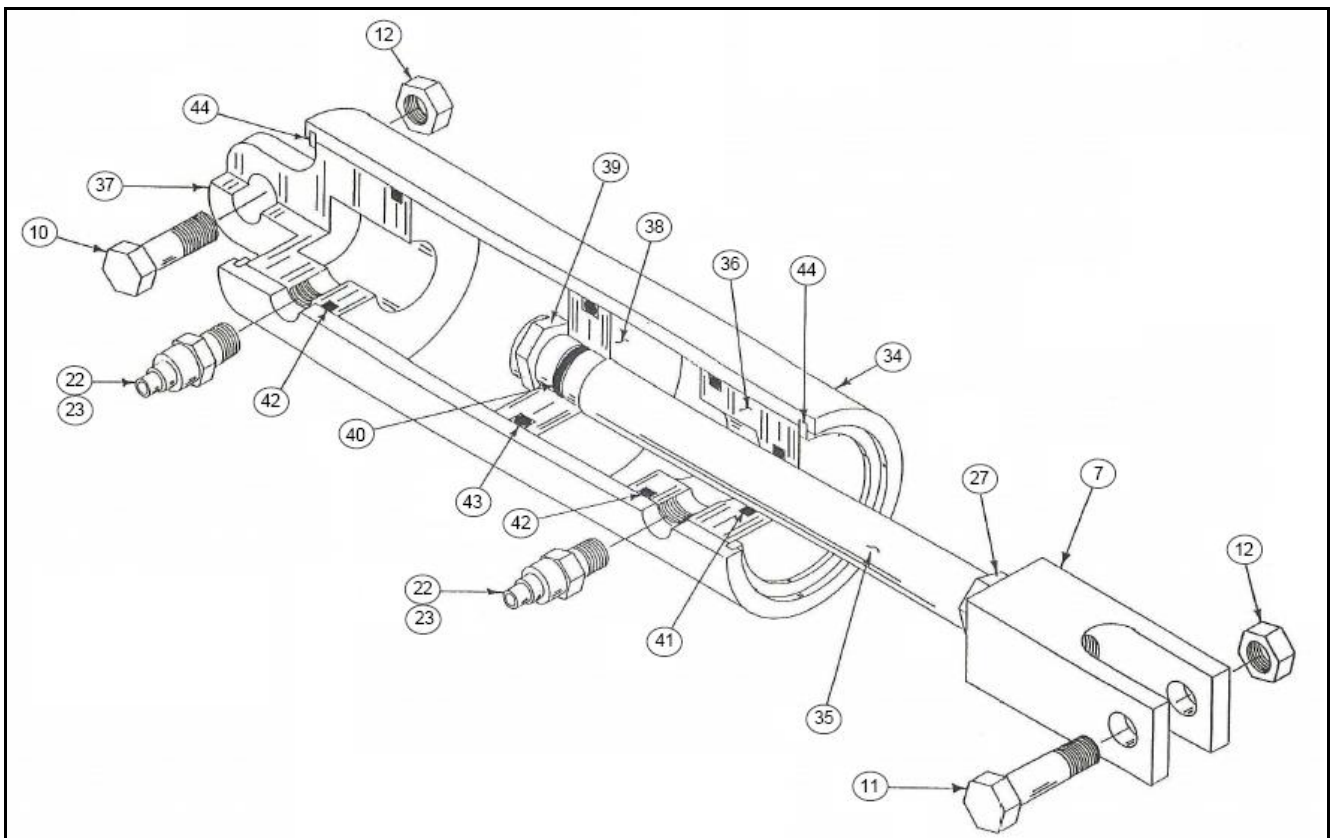
Figure 2: Pneumatic Cylinder Parts
