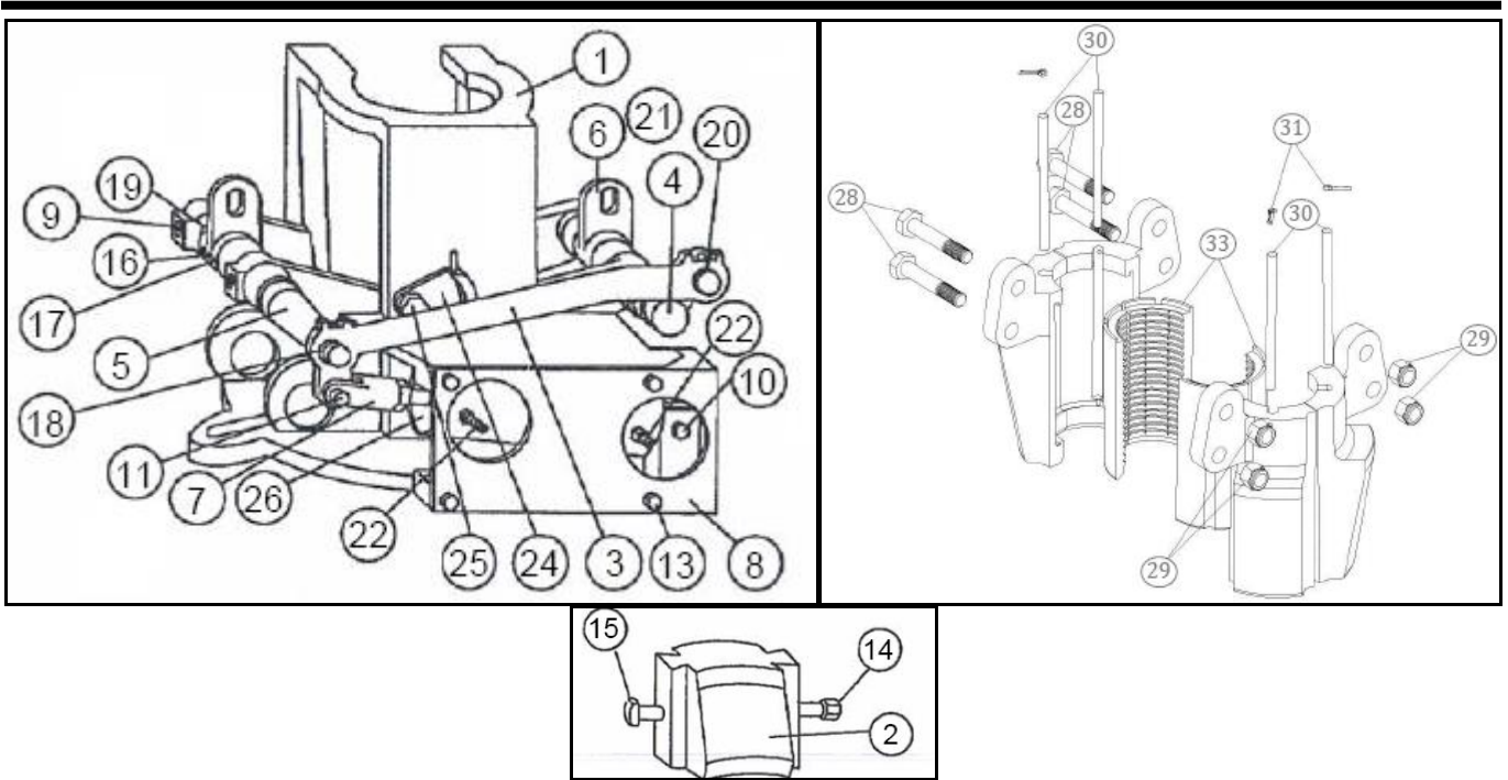
Figure 1: Tubing Spider Parts
